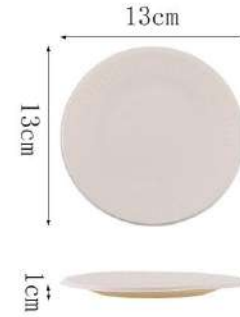
MDS05-02 Biodegradable 5' plate
